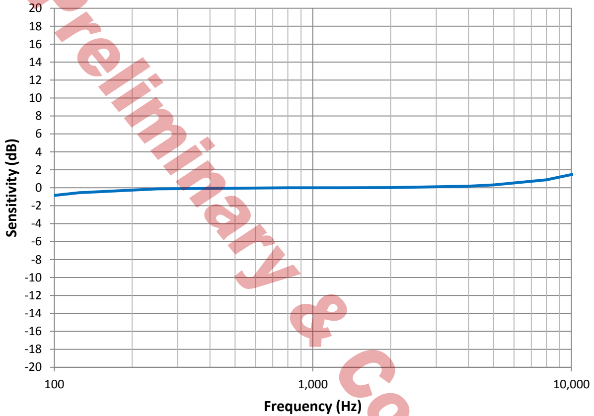
Typical Free Field Response Normalized to 1 kHz
